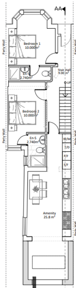
Ground floor Including 3m permitted development rear extension to replace 2.2m conservatory
