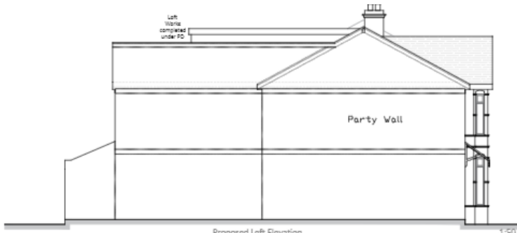
Proposed Left Elevation 1:50
