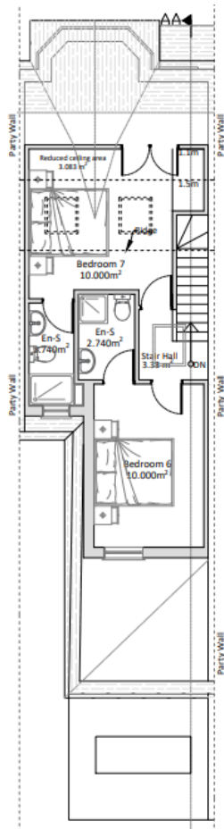
Second floor
