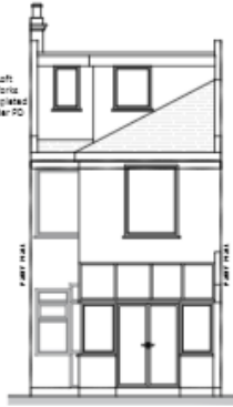
Proposed Rear Elevation 1:50
