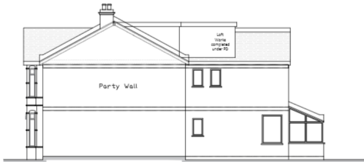
Proposed Right Elevation 1:50
