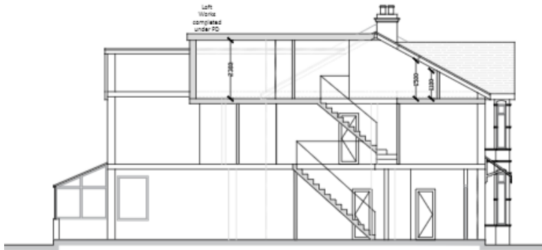
Proposed Section AA 1:50
