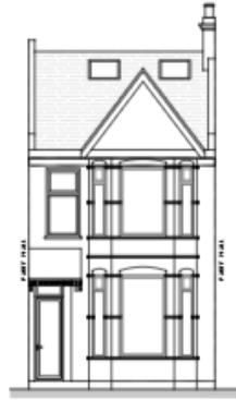
Proposed Front Elevation 1:50
